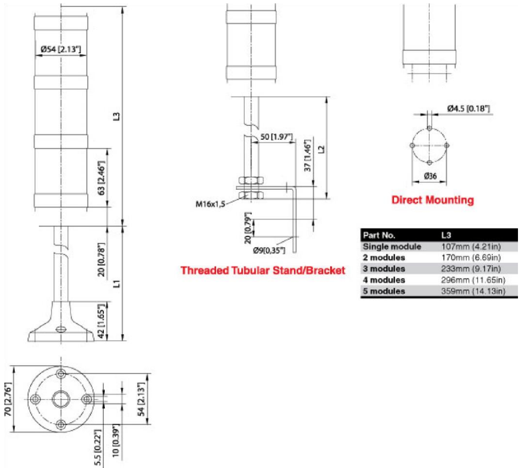
Tubular Stand/Plinth
